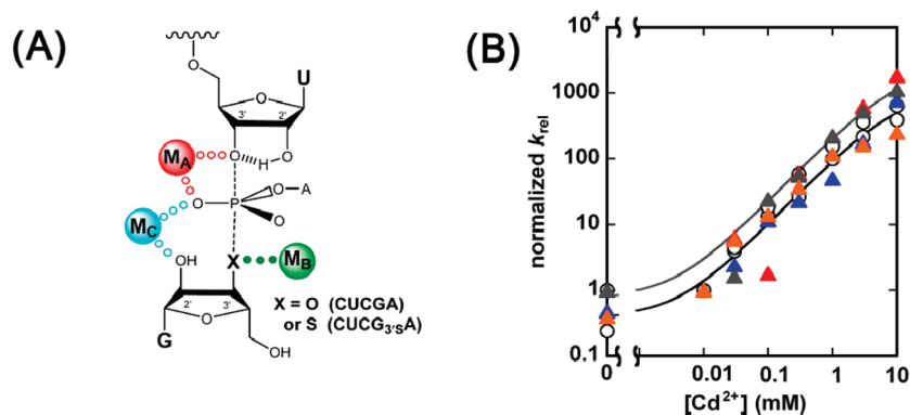
FIGURE 5: M_B rescue of CUCG 3' SA cleavage for wild-type and modified ribozymes. Rescue reactions were carried out as indicated in the text and in Materials and Methods. (A) The metal ion–substrate contact being probed is indicated by green solid dots in the model for the Tetrahymena ribozyme transition state. X represents an oxygen or sulfur atom in the guanosine analogues CUCGA and CUCG 3' SA, respectively. (B) Rescue profiles for the wt (○), C208S P (red △), A304S P (blue △), A306S P (gray △), and U307S P (orange △) ribozymes. k_{rel} represents the observed rate constant for cleavage of CUCG 3' SA relative to CUCGA and was normalized to equal 1 in the absence of Cd^{2+} .
