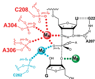
FIGURE 7: Proposed model of the Tetrahymena ribozyme transition state from functional data (ref 10 and references cited therein and this work). Bonds made and broken at the transition state are represented by dashed lines. Hydrogen bonds are represented by hashed lines. Functional contacts between metal ions and their ligands are represented by solid dots of the same color of the metal ion; contacts from this work are in larger font.
