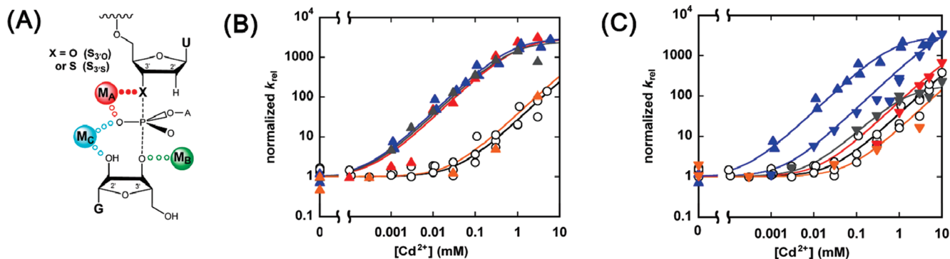
FIGURE 4: M A rescue of S 3'S cleavage for wild-type and modified ribozymes. Cd 2+ rescue reactions were carried out as indicated in the text and in Materials and Methods. (A) The metal ion–substrate contact being probed is indicated by solid dots in the model for the Tetrahymena ribozyme transition state. X represents an oxygen or sulfur atom in the oligonucleotide substrates S 3'O and S 3'S , respectively. (B) Rescue profiles for the wt (○), C208S P (red △), A304S P (blue △), A306S P (gray △), and U307S P (orange △) ribozymes. (C) Rescue profiles for the wt (○), C208R P (red ▽), A304R P (blue ▽), A306R P (gray ▽), and U307R P (orange ▽) ribozymes. The rescue profile of the A304S P ribozyme (blue △) is repeated from panel B to aid comparison. k rel represents the observed rate constant for cleavage of S 3'S relative to S 3'O and was normalized to equal 1 in the absence Cd 2+ .
